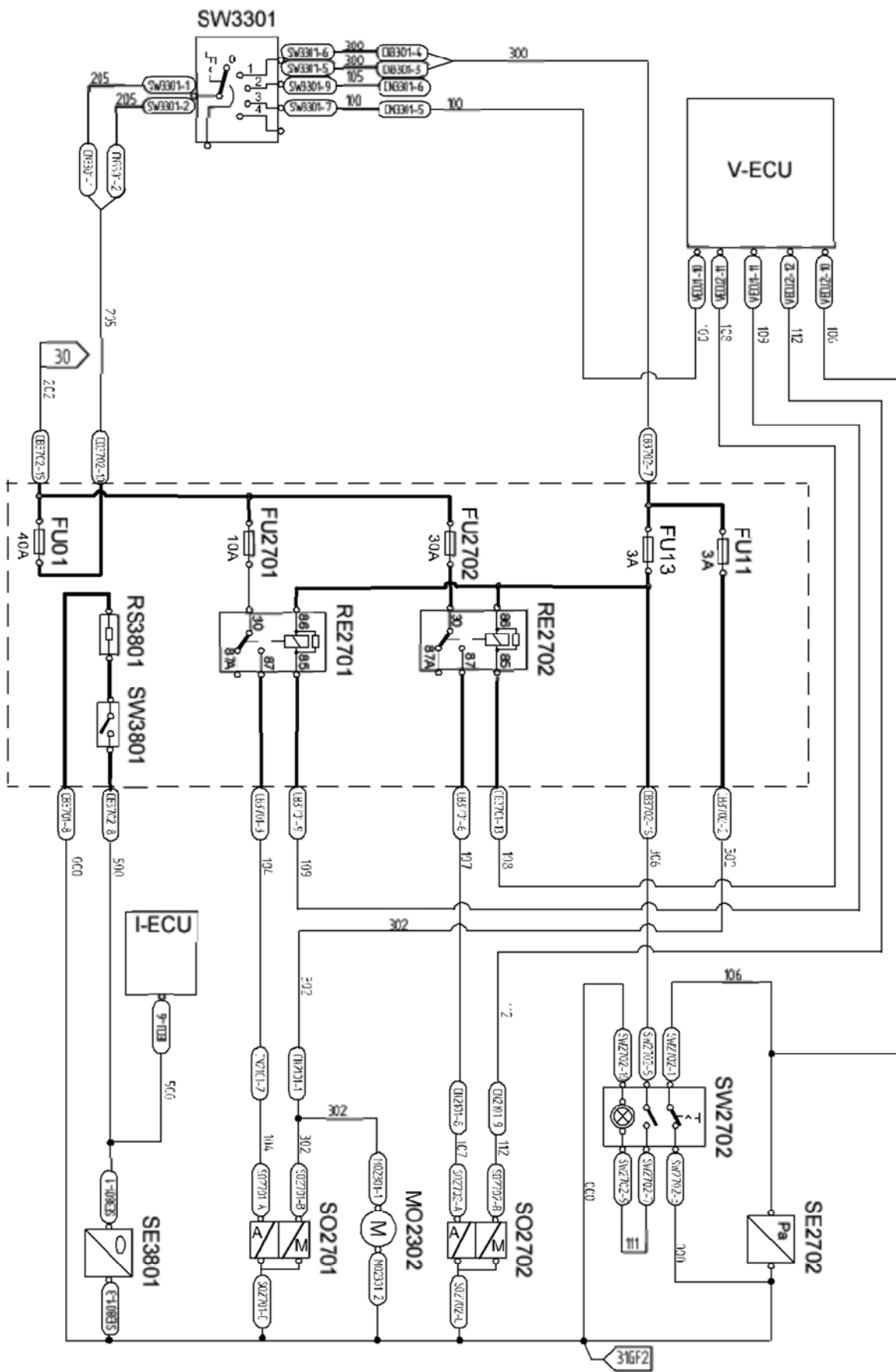
Figure 2 Fuel circuit
